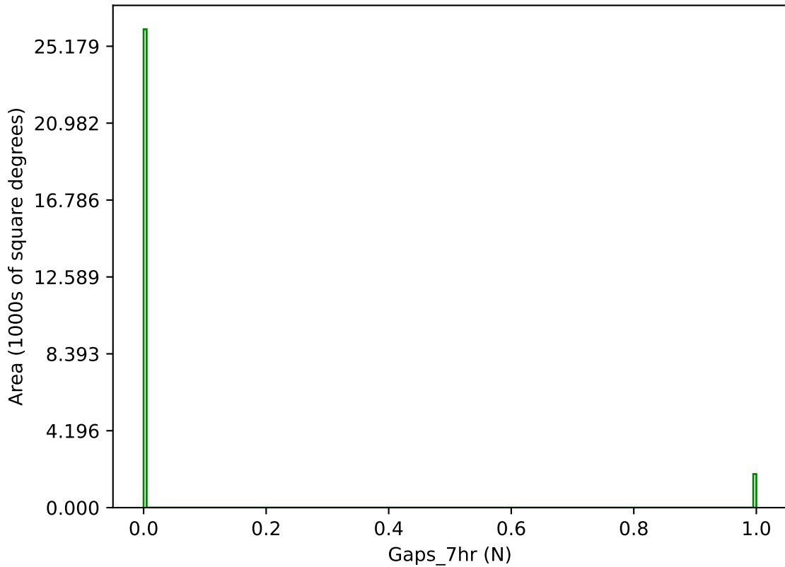
ddf_loaded_fl4_v3.4_10yrs g band: Gaps_7hr
