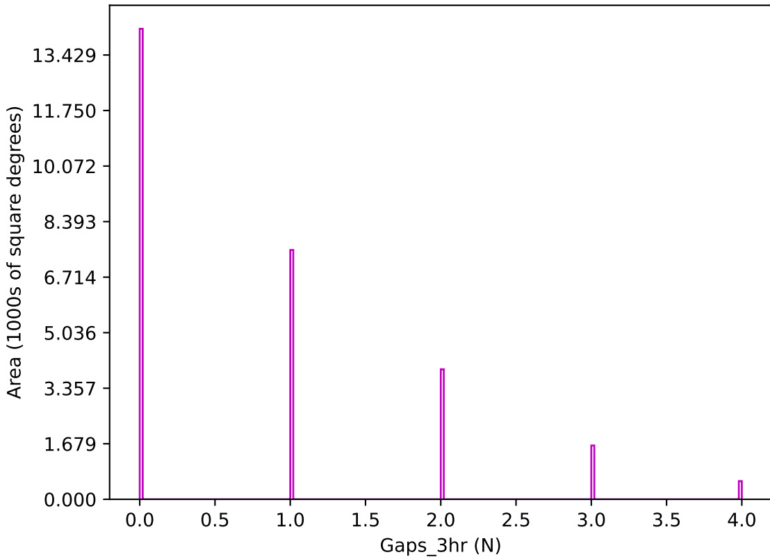
ddf_loaded_fl4_v3.4_10yrs z band: Gaps_3hr
