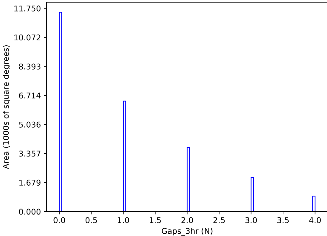
ddf_loaded_fl4_v3.4_10yrs y band: Gaps_3hr
