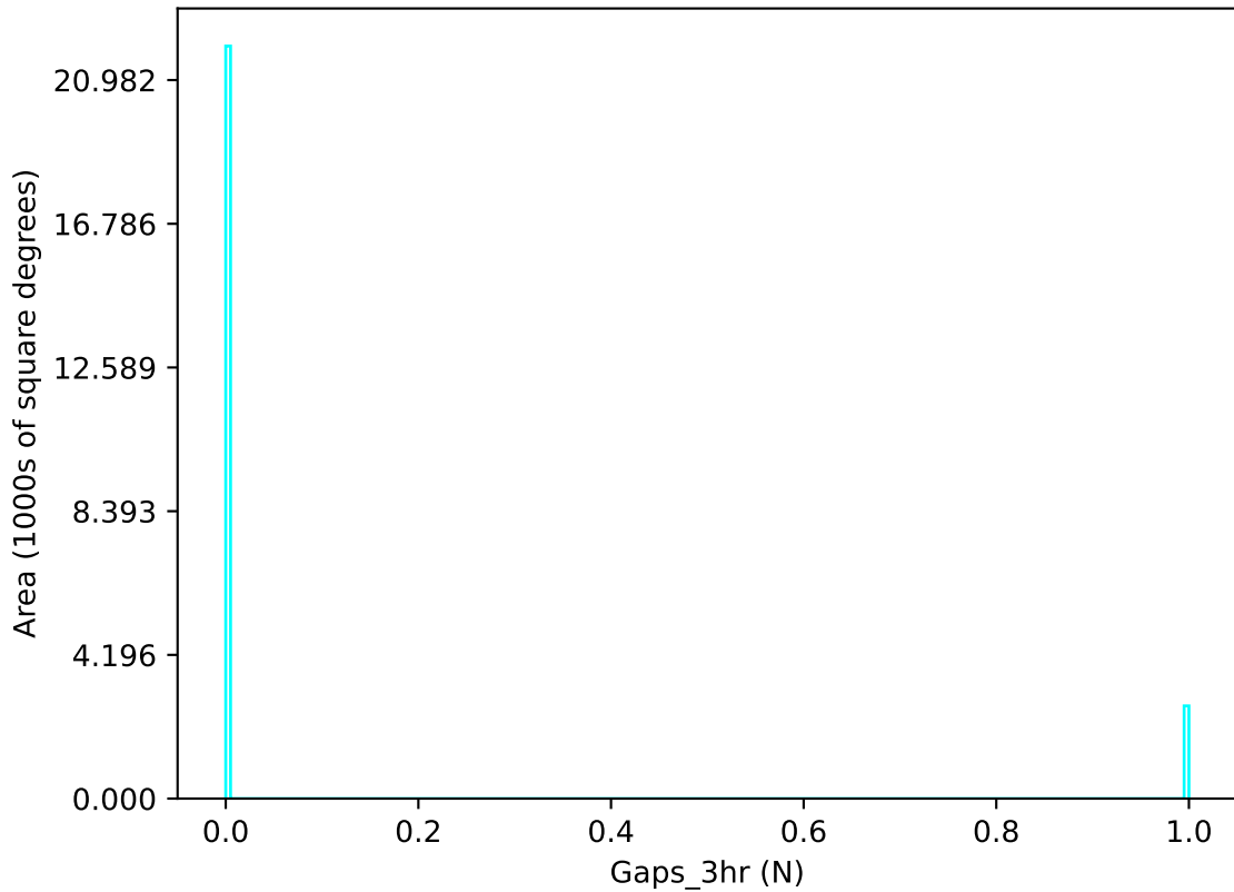
ddf_loaded_fl4_v3.4_10yrs u band: Gaps_3hr
