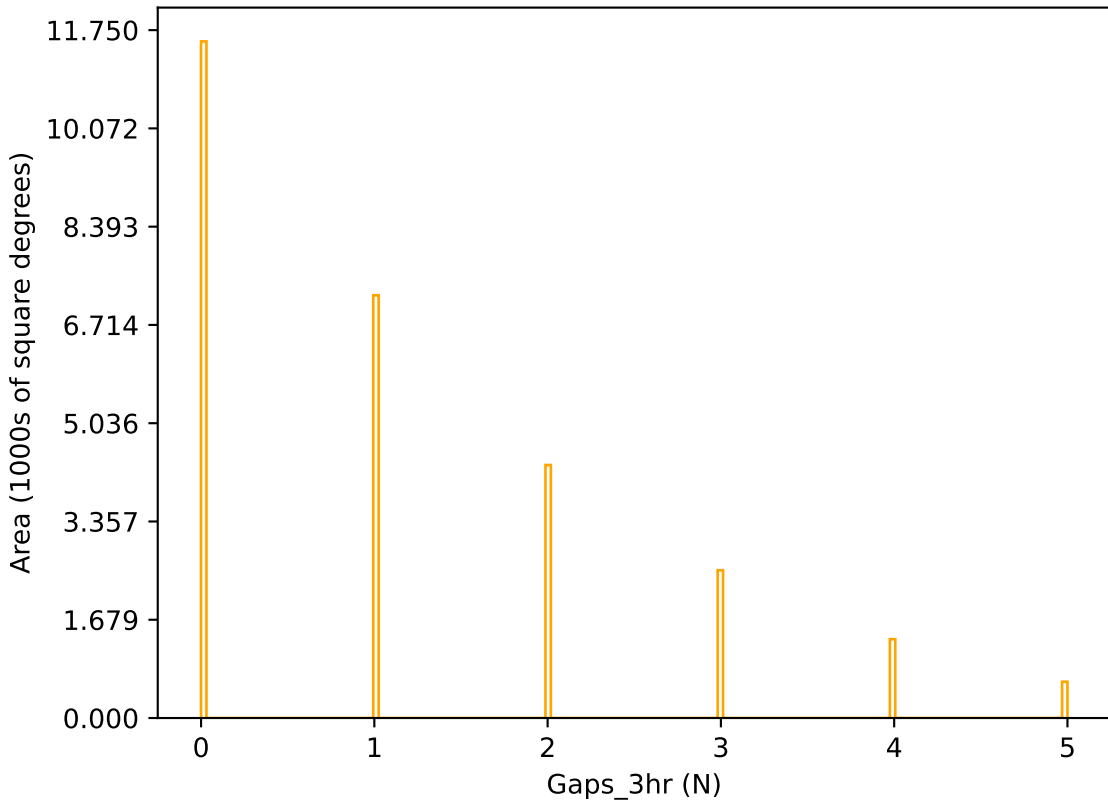
ddf_loaded_fl4_v3.4_10yrs r band: Gaps_3hr
