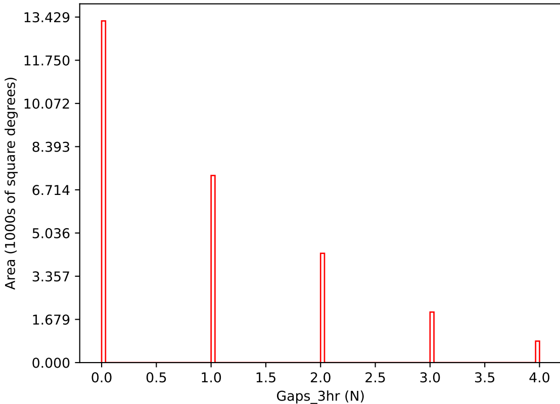
ddf_loaded_fl4_v3.4_10yrs i band: Gaps_3hr
