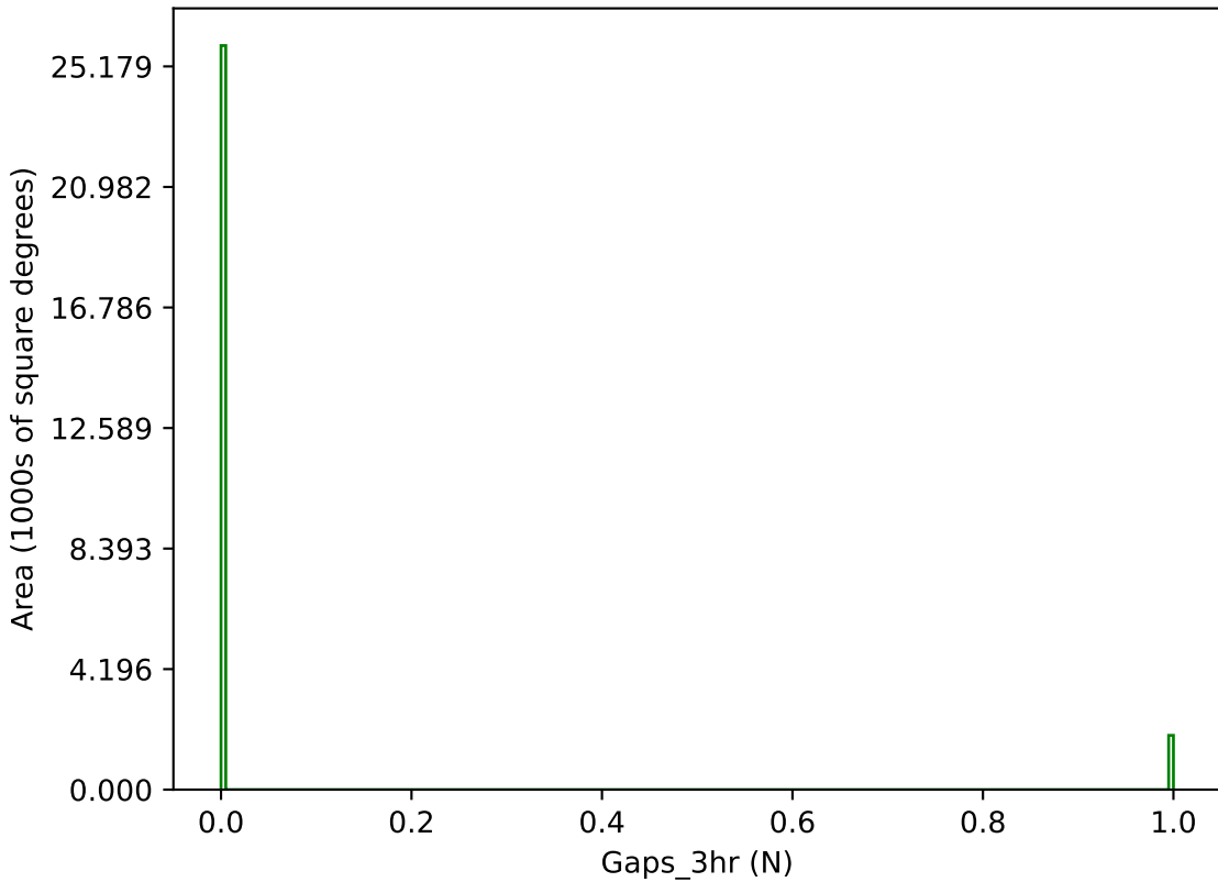
ddf_loaded_fl4_v3.4_10yrs g band: Gaps_3hr
