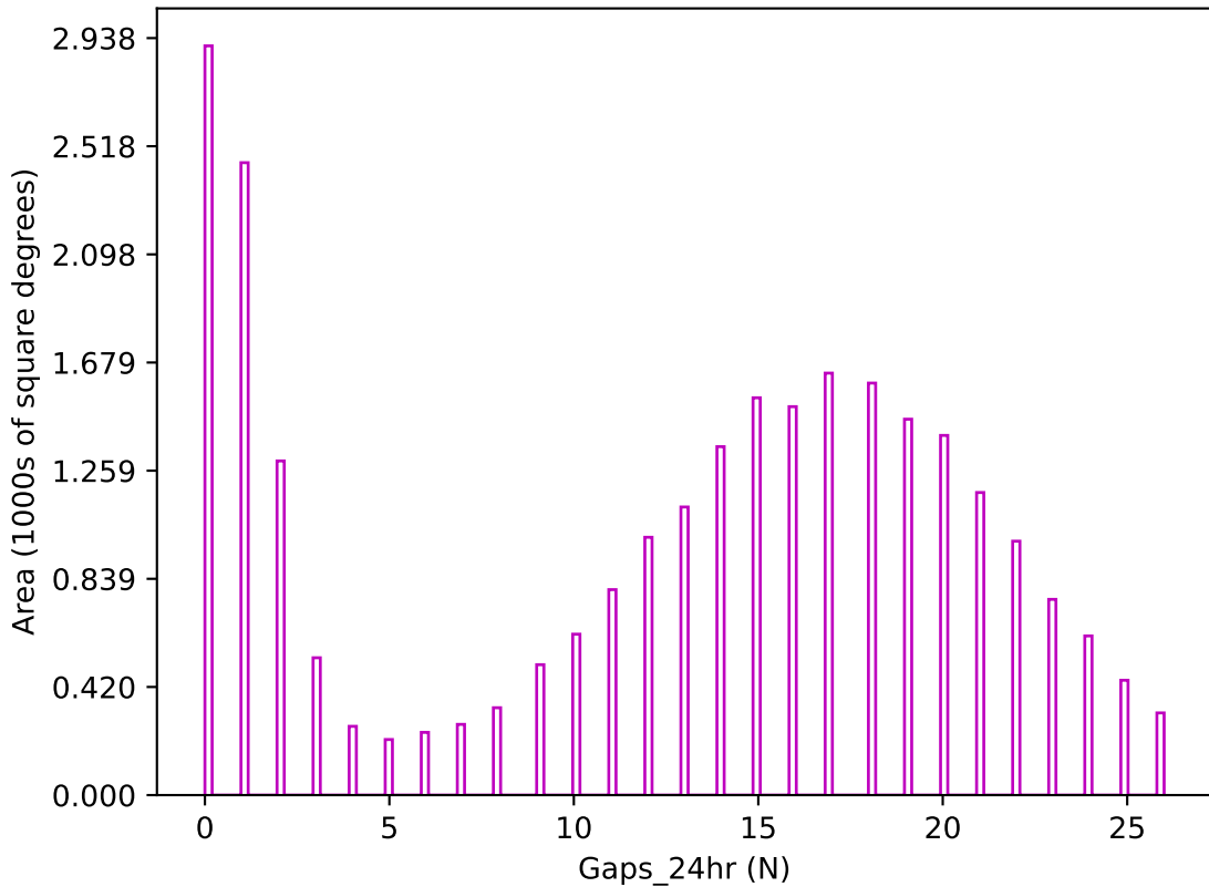
ddf_loaded_fl4_v3.4_10yrs z band: Gaps_24hr
