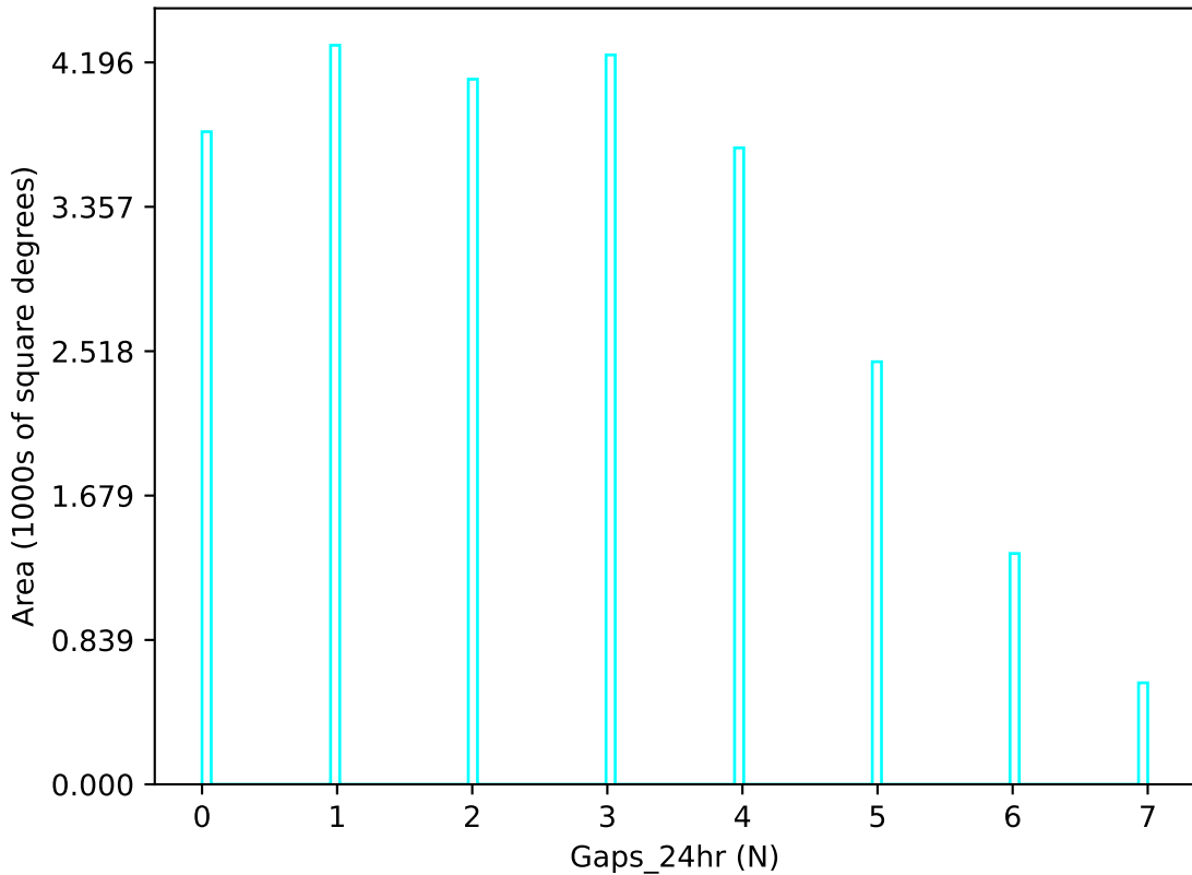
ddf_loaded_fl4_v3.4_10yrs u band: Gaps_24hr
