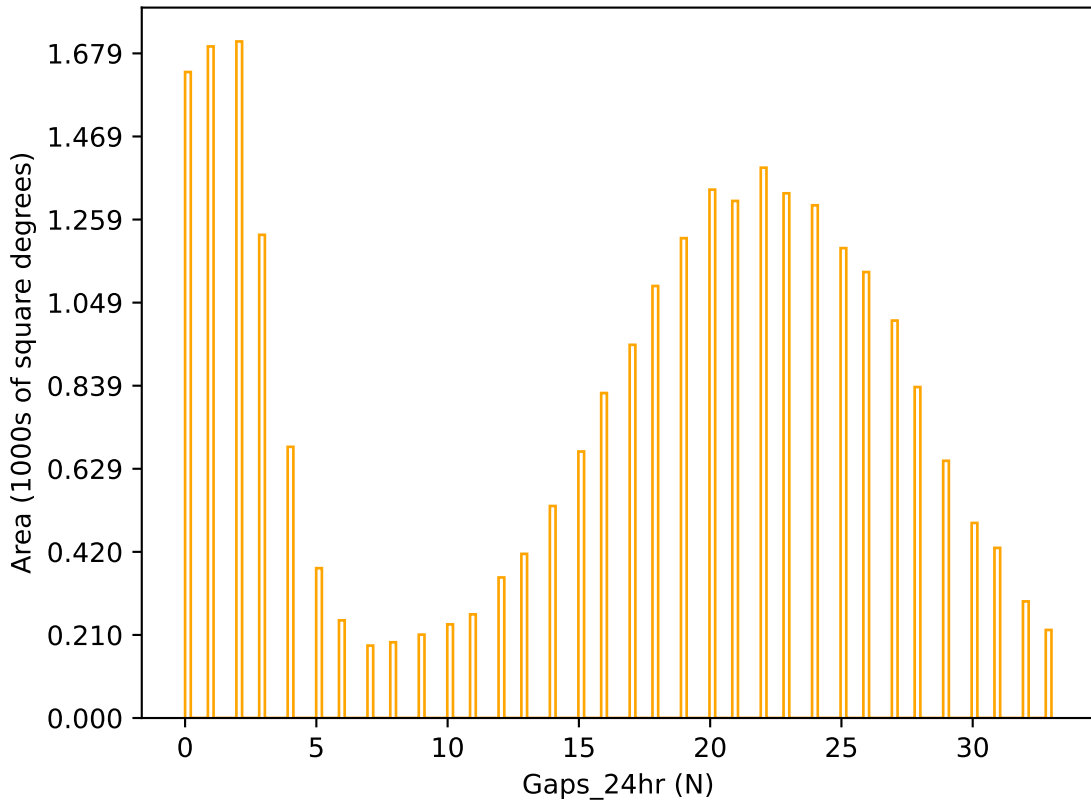
ddf_loaded_fl4_v3.4_10yrs r band: Gaps_24hr
