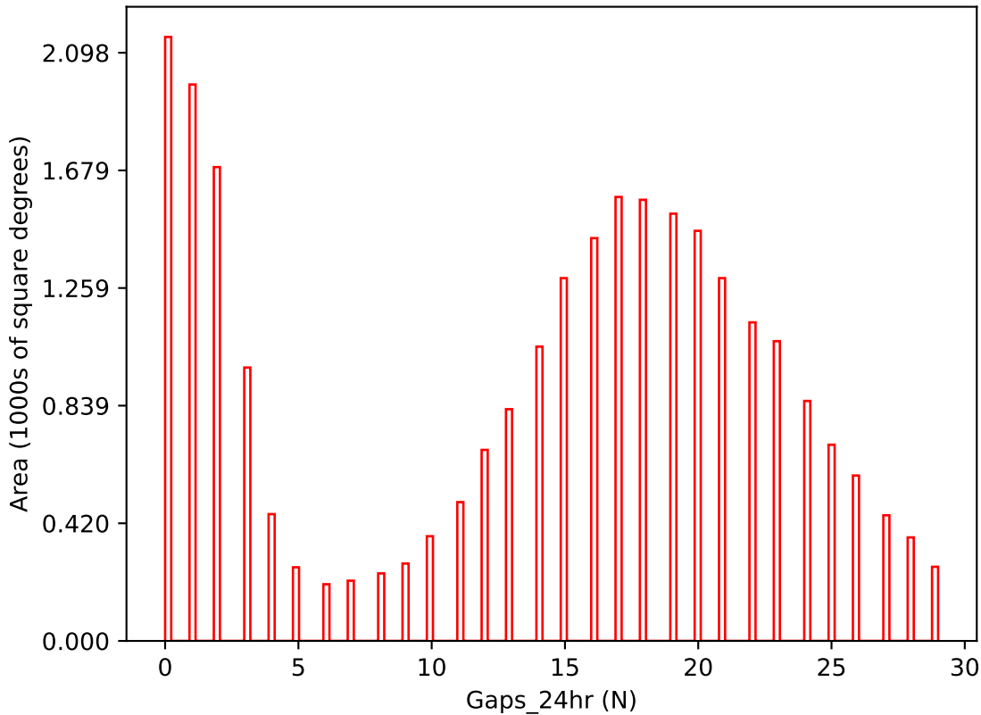
ddf_loaded_fl4_v3.4_10yrs i band: Gaps_24hr
