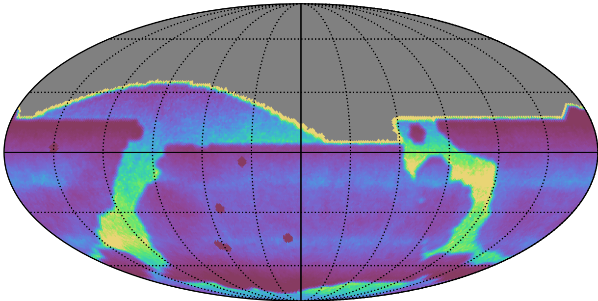
ddf_loaded_fl4_v3.4_10yrs : DCRprecision
