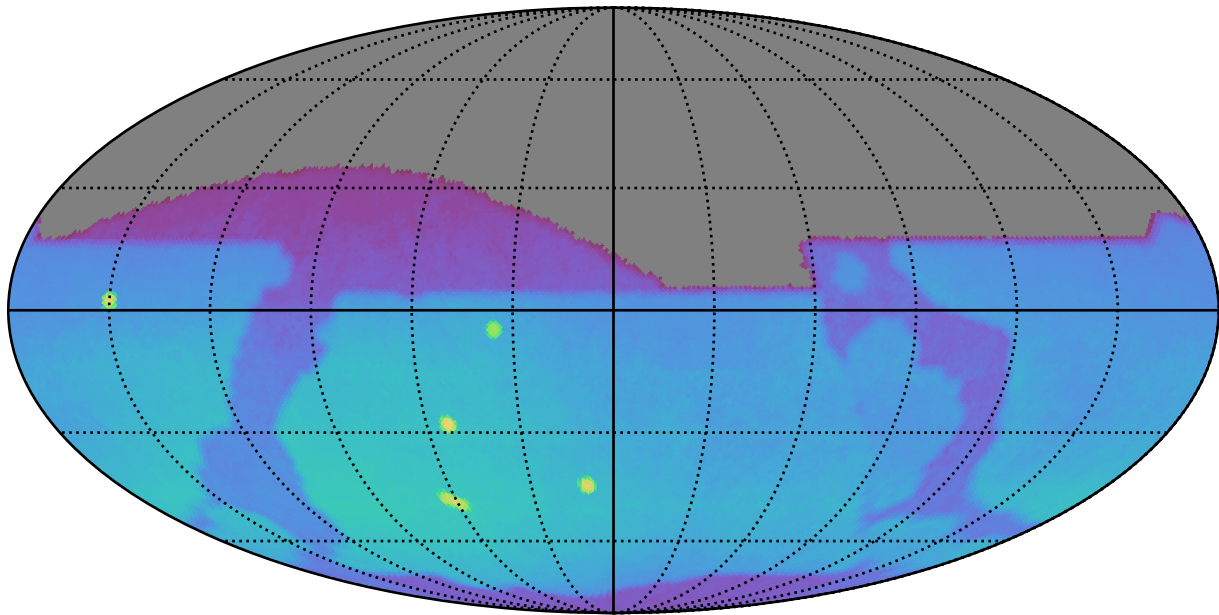
ddf_loaded_fl4_v3.4_10yrs : Brown Dwarf, L7
