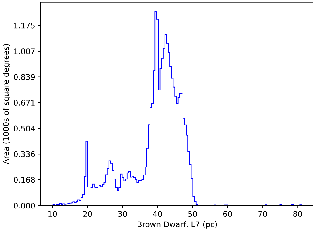
ddf_loaded_fl4_v3.4_10yrs : Brown Dwarf, L7
