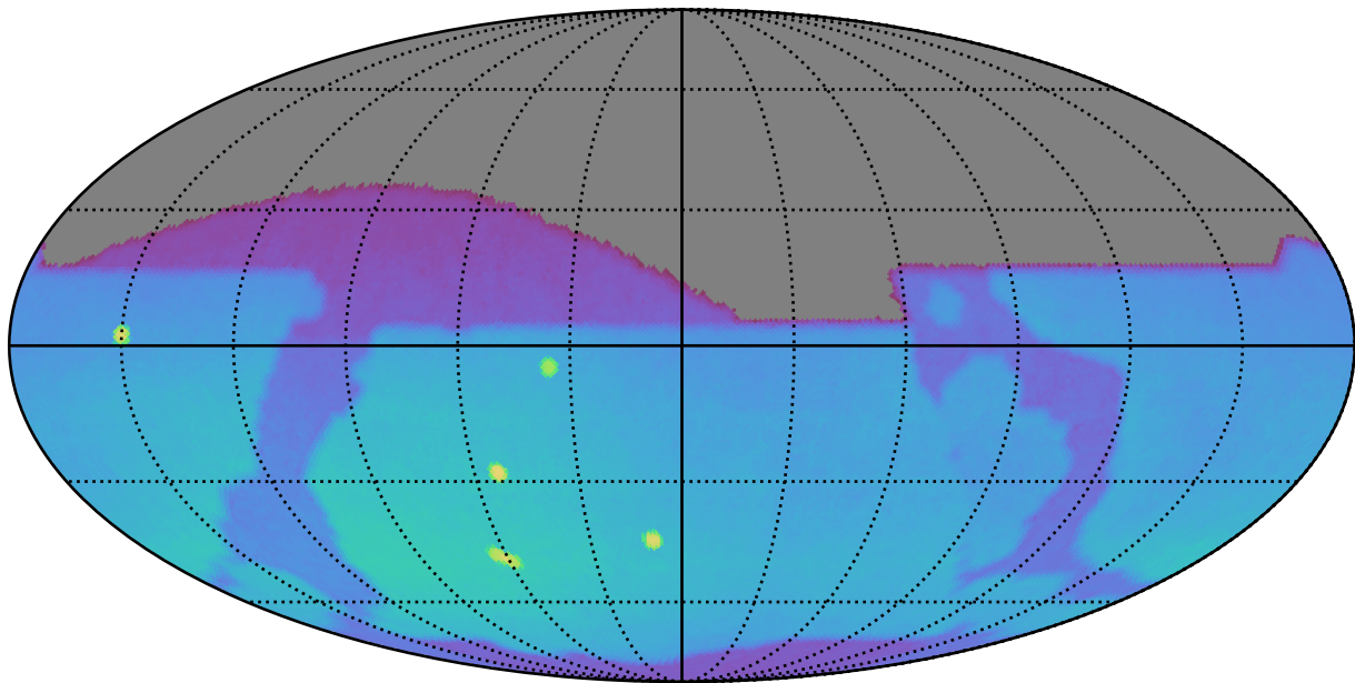
ddf_loaded_fl4_v3.4_10yrs : Brown Dwarf, L4
