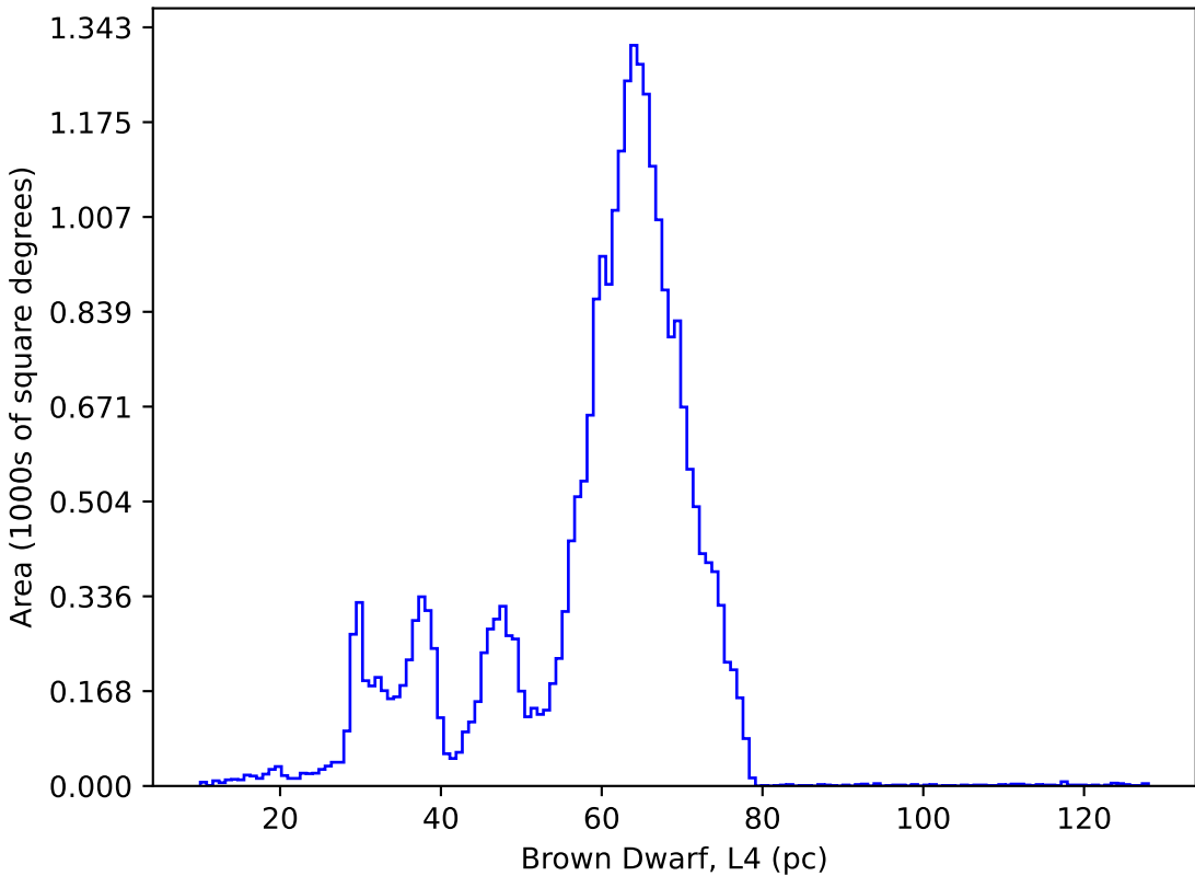
ddf_loaded_fl4_v3.4_10yrs : Brown Dwarf, L4
