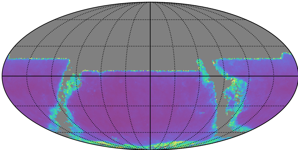
ddf_loaded_fl4_v3.4_10yrs y band: AGN SF_uncert
