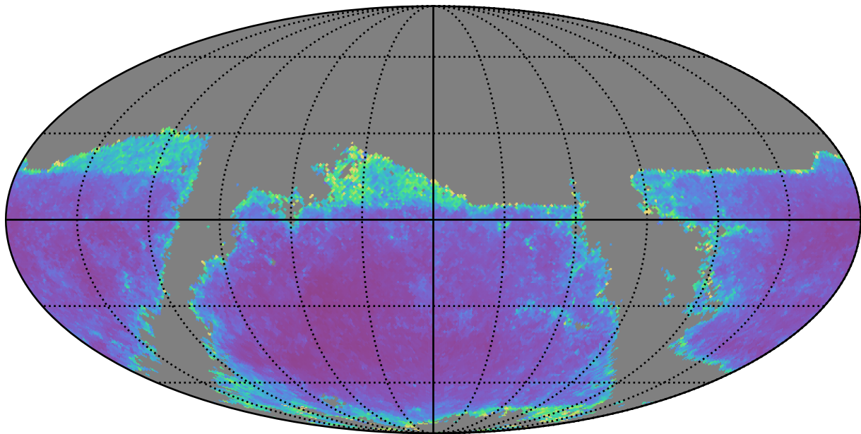
ddf_loaded_fl4_v3.4_10yrs g band: AGN SF_uncert
