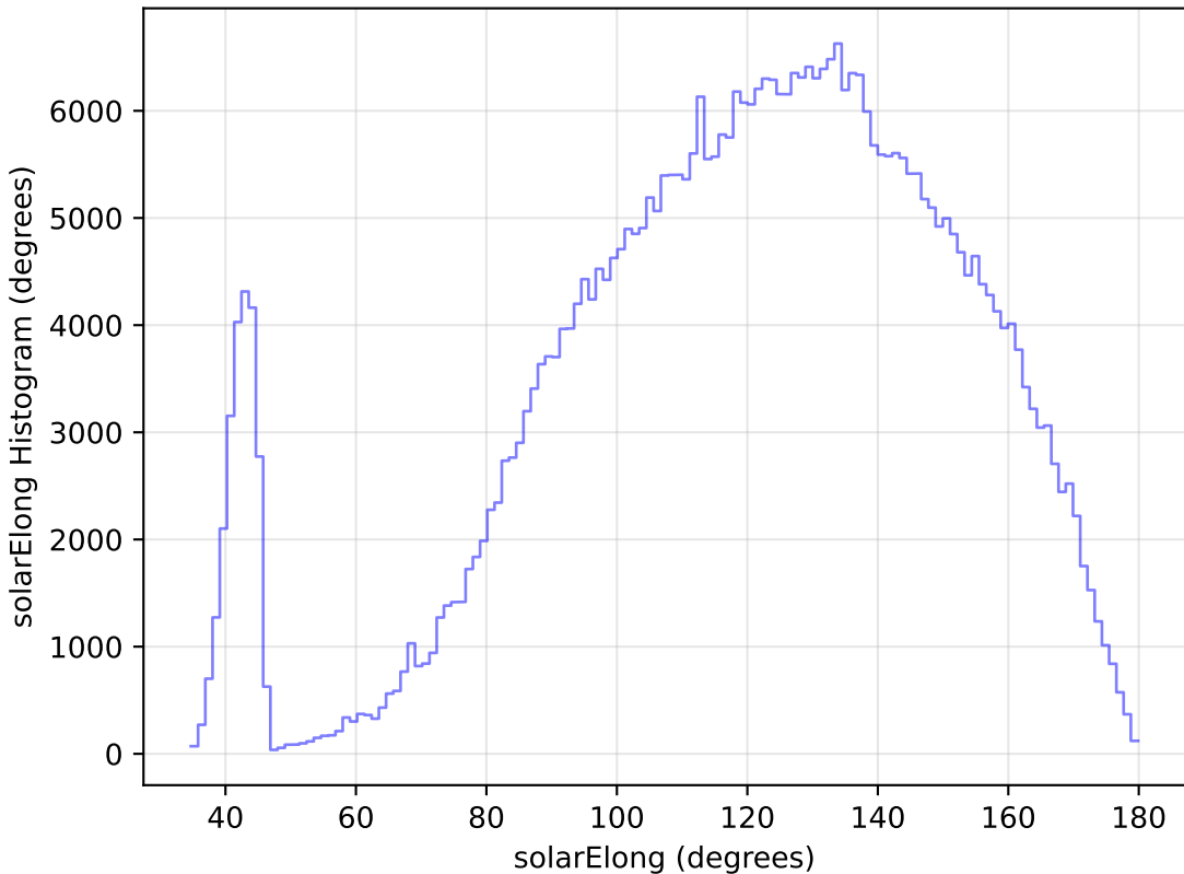
ddf_loaded_fl4_v3.4_10yrs WFD z band: solarElong Histogram
