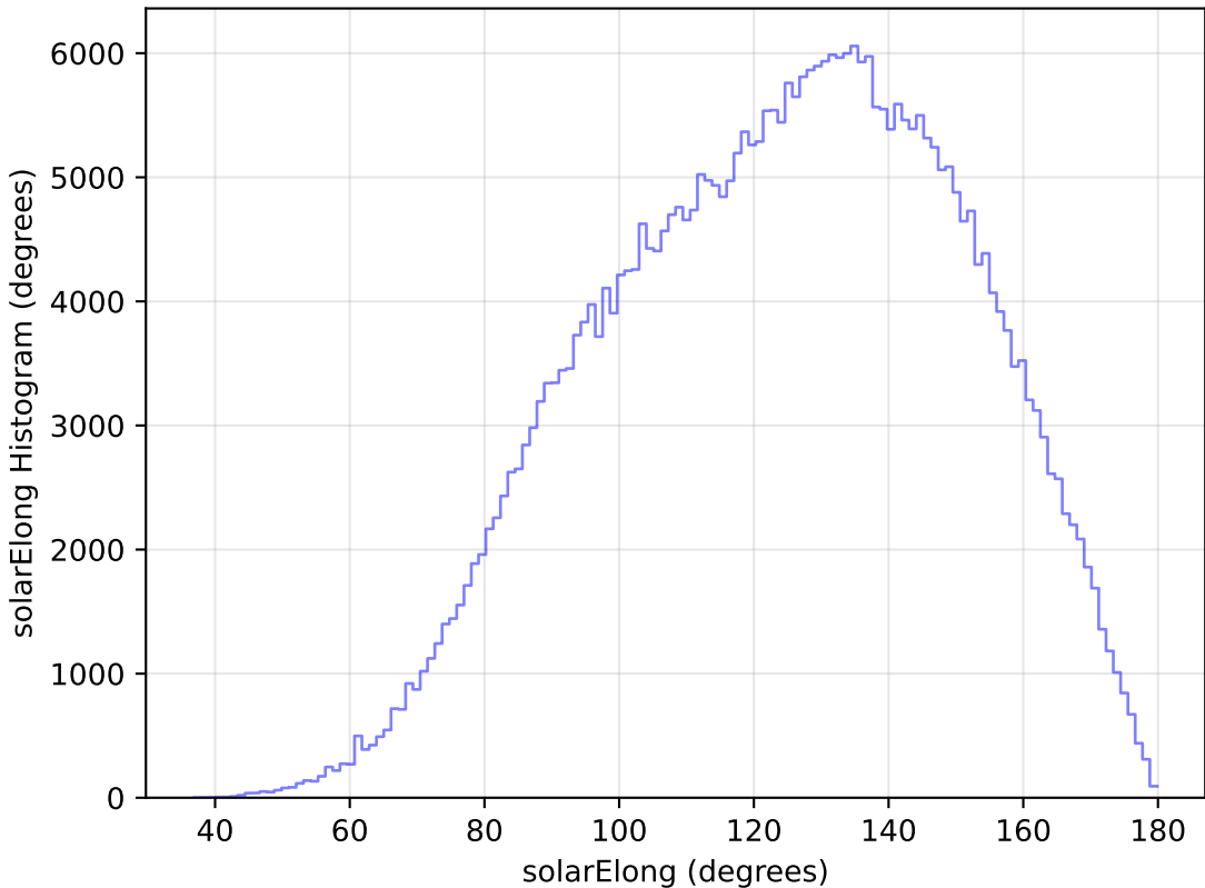
ddf_loaded_fl4_v3.4_10yrs WFD y band: solarElong Histogram
