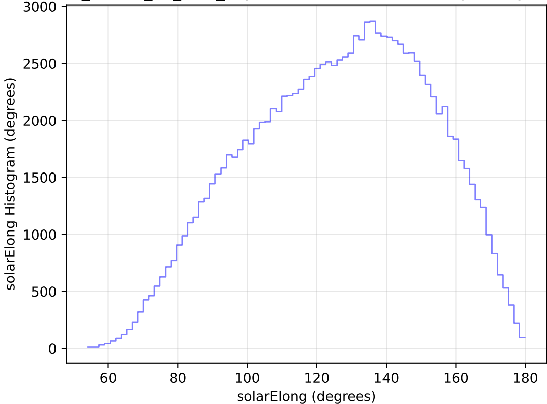
ddf_loaded_fl4_v3.4_10yrs WFD u band: solarElong Histogram
