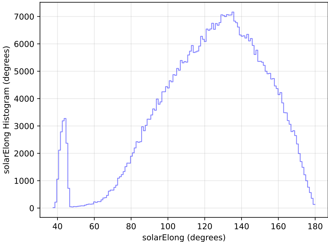
ddf_loaded_fl4_v3.4_10yrs WFD r band: solarElong Histogram
