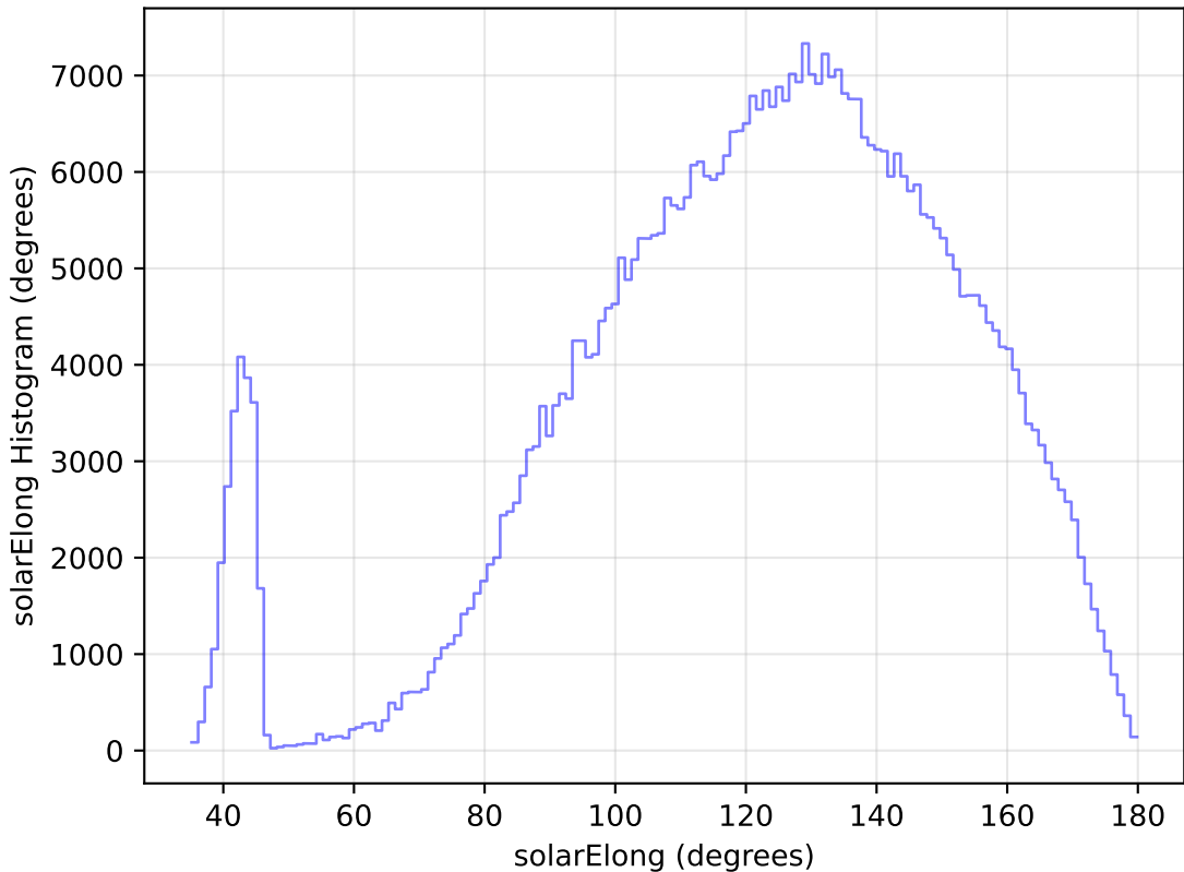
ddf_loaded_fl4_v3.4_10yrs WFD i band: solarElong Histogram
