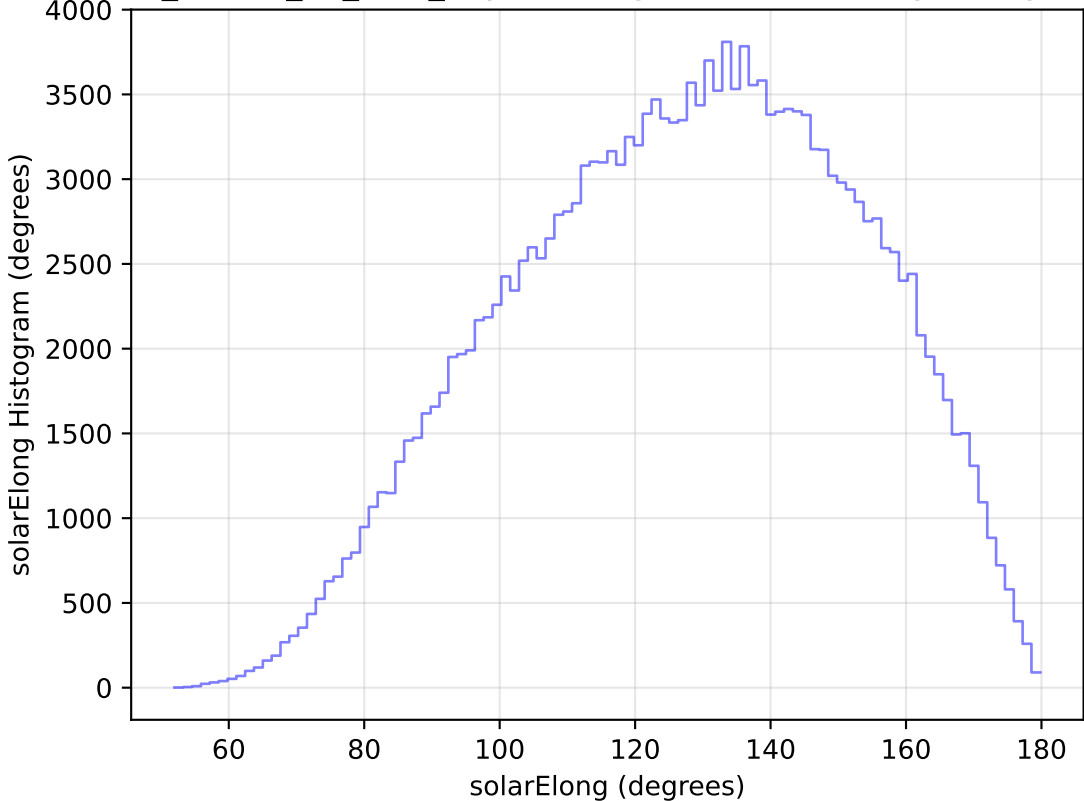
ddf_loaded_fl4_v3.4_10yrs WFD g band: solarElong Histogram
