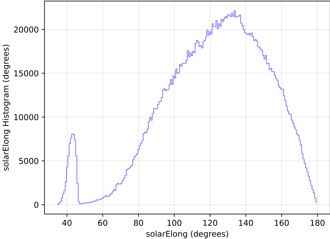
ddf_loaded_fl4_v3.4_10yrs WFD all bands: solarElong Histogram
