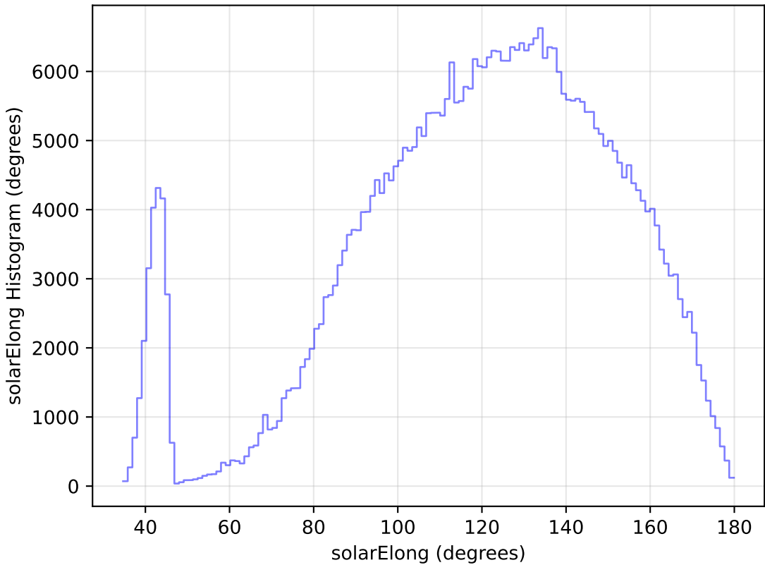
ddf_loaded_fl4_v3.4_10yrs All sky z band: solarElong Histogram
