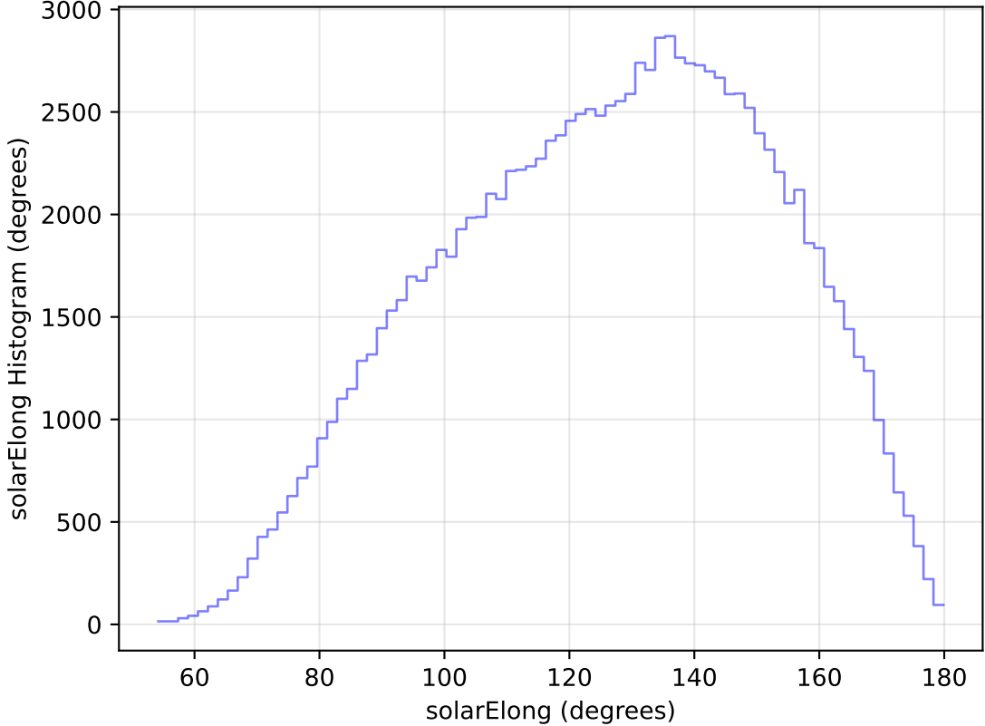
ddf_loaded_fl4_v3.4_10yrs All sky u band: solarElong Histogram
