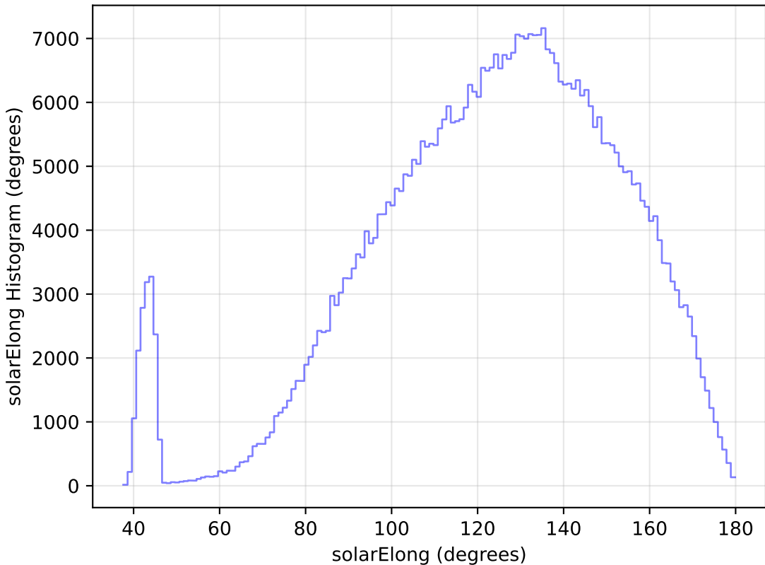
ddf_loaded_fl4_v3.4_10yrs All sky r band: solarElong Histogram
