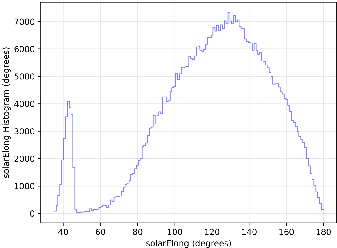
ddf_loaded_fl4_v3.4_10yrs All sky i band: solarElong Histogram
