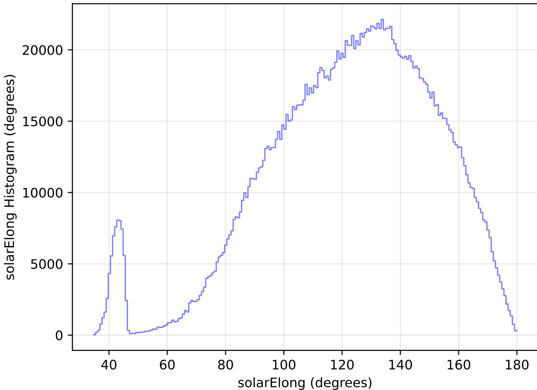
ddf_loaded_fl4_v3.4_10yrs All sky all bands: solarElong Histogram
