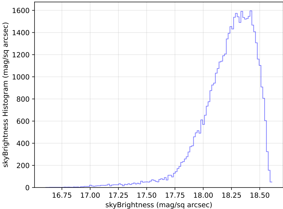
ddf_loaded_fl4_v3.4_10yrs Yr 1 y band: skyBrightness Histogram
