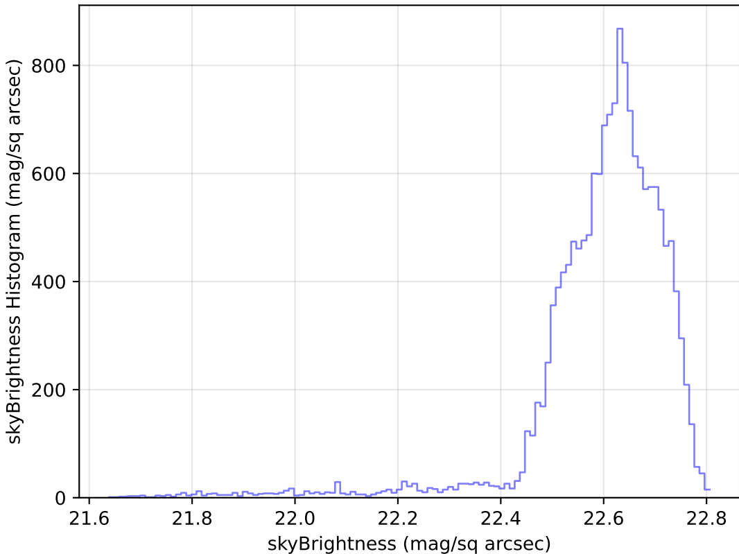
ddf_loaded_fl4_v3.4_10yrs Yr 1 u band: skyBrightness Histogram
