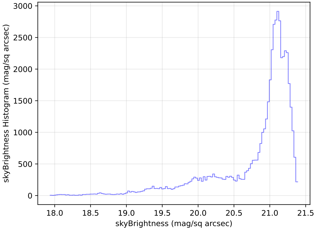
ddf_loaded_fl4_v3.4_10yrs Yr 1 r band: skyBrightness Histogram
