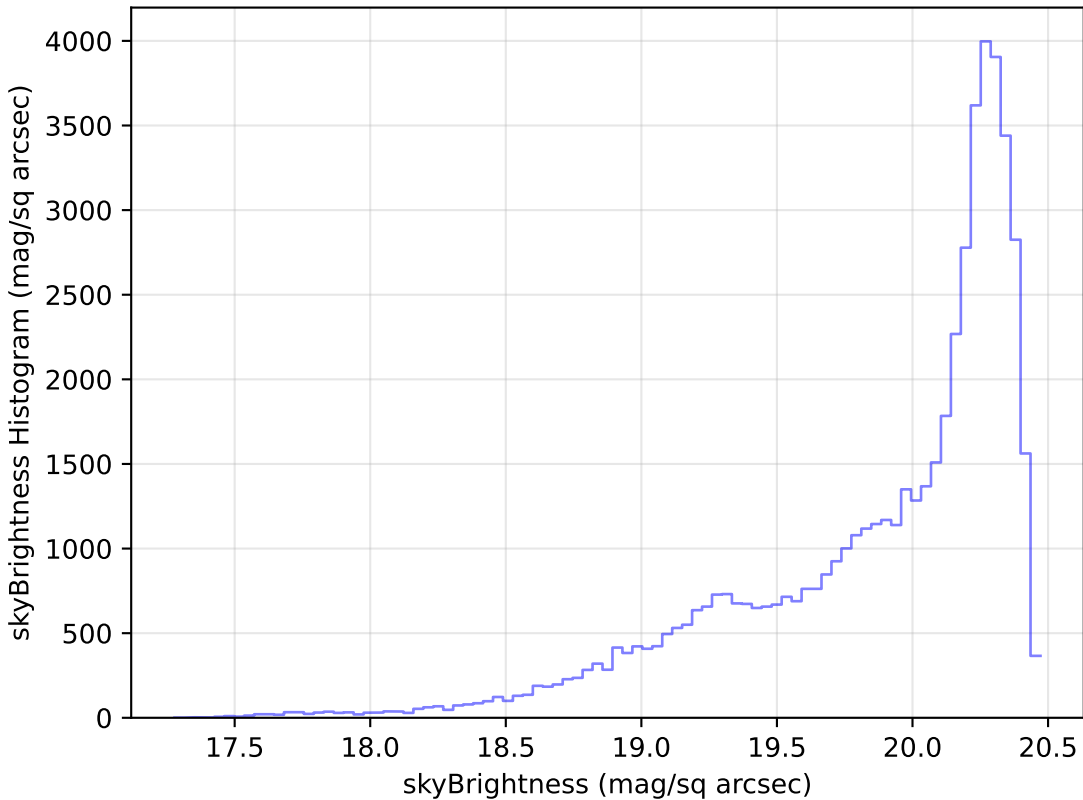
ddf_loaded_fl4_v3.4_10yrs Yr 1 i band: skyBrightness Histogram
