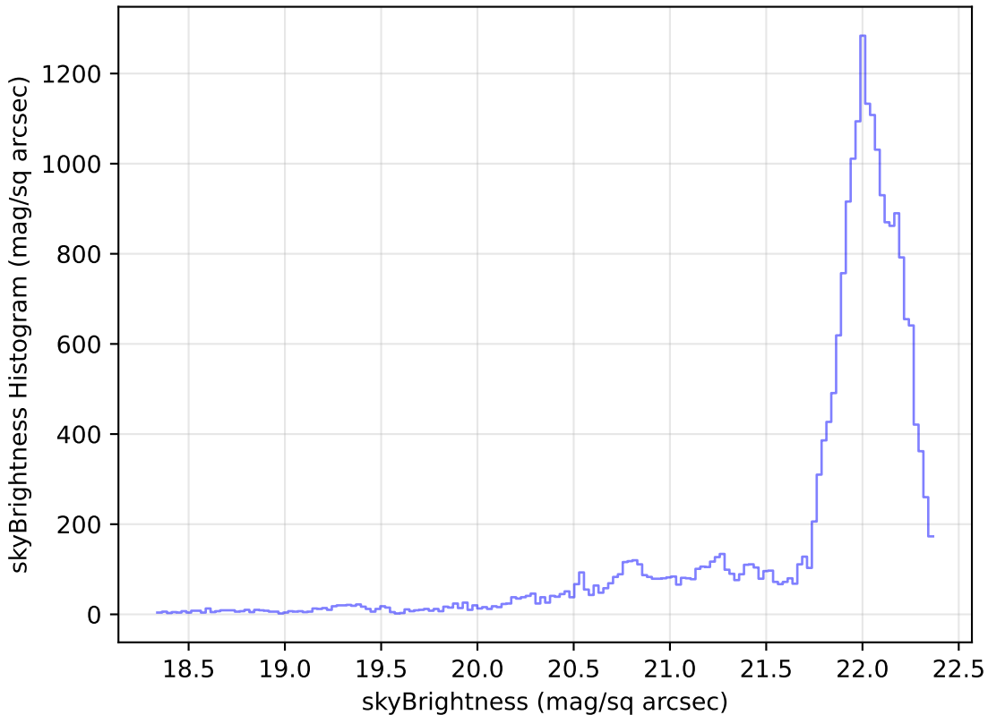
ddf_loaded_fl4_v3.4_10yrs Yr 1 g band: skyBrightness Histogram
