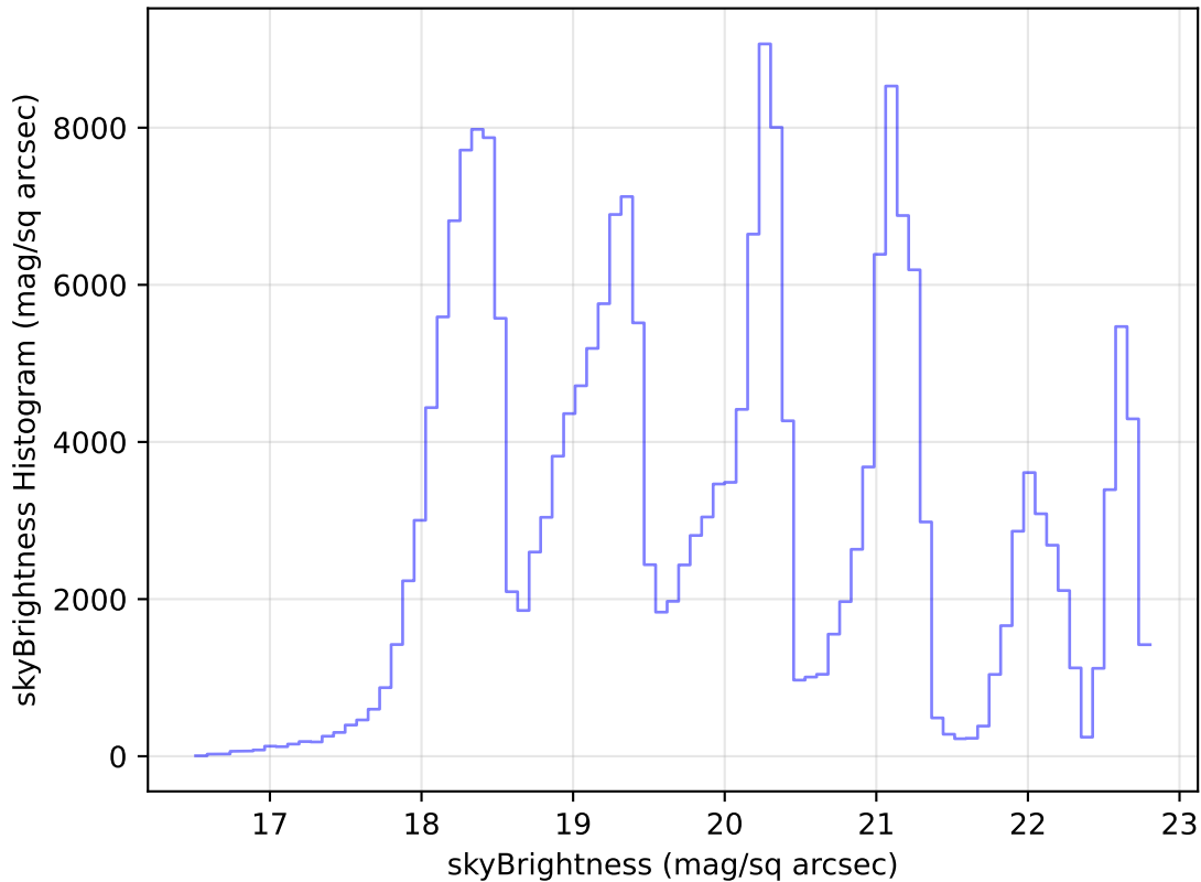
ddf_loaded_fl4_v3.4_10yrs Yr 1 all bands: skyBrightness Histogram
