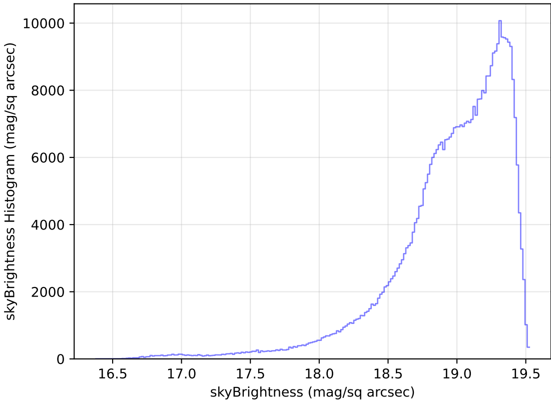
ddf_loaded_fl4_v3.4_10yrs WFD z band: skyBrightness Histogram
