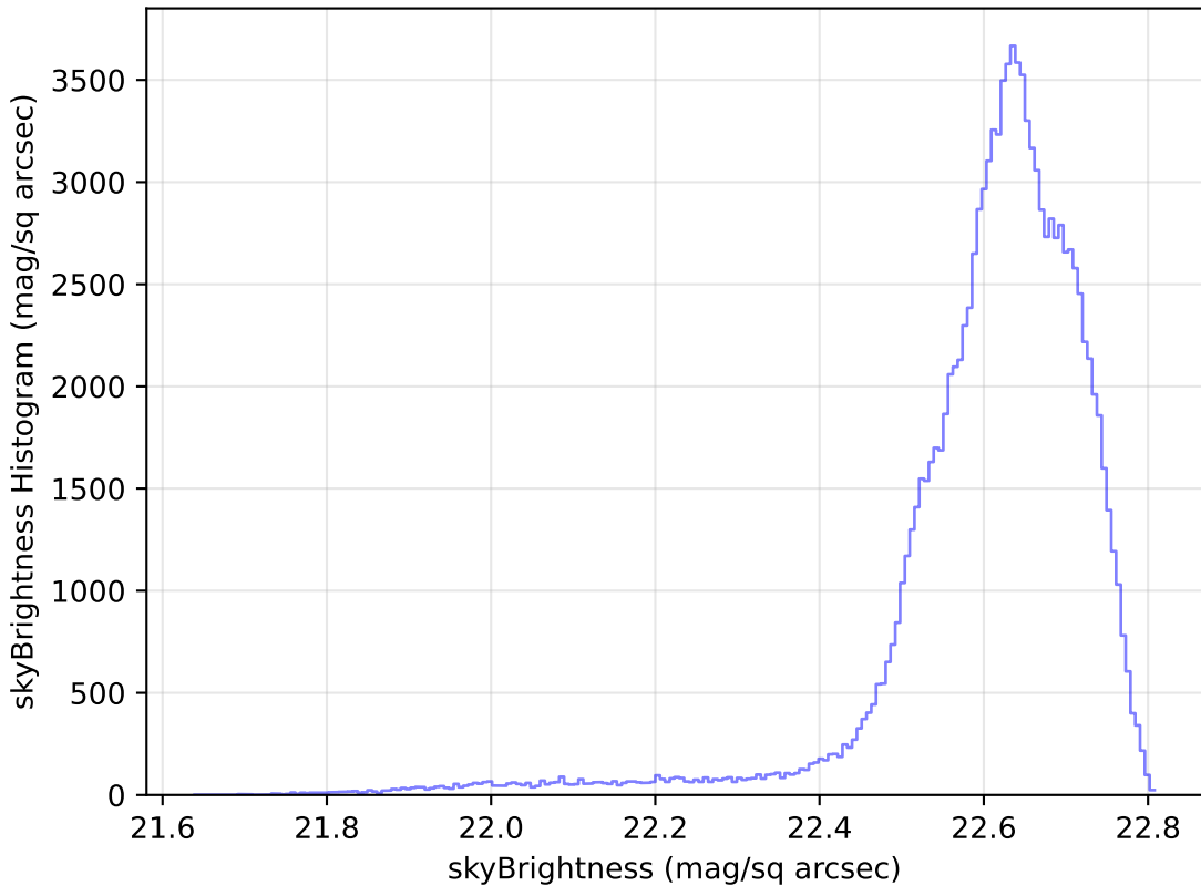
ddf_loaded_fl4_v3.4_10yrs WFD u band: skyBrightness Histogram
