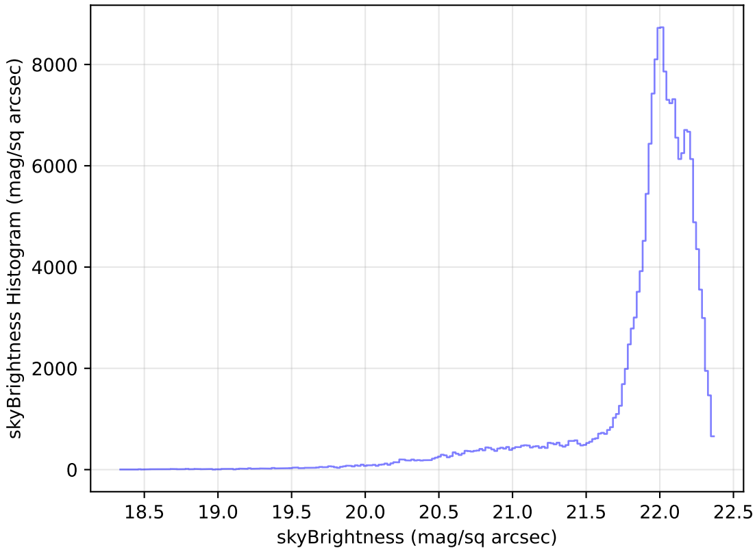
ddf_loaded_fl4_v3.4_10yrs WFD g band: skyBrightness Histogram
