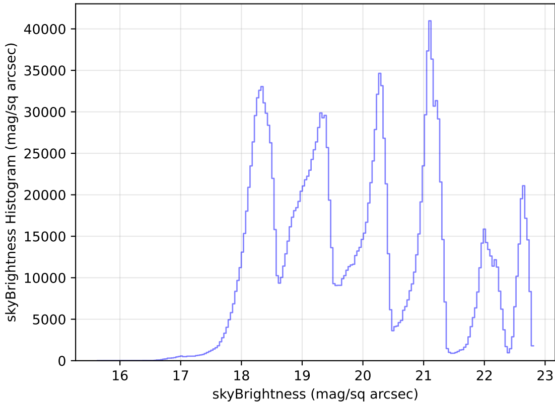
ddf_loaded_fl4_v3.4_10yrs WFD all bands: skyBrightness Histogram
