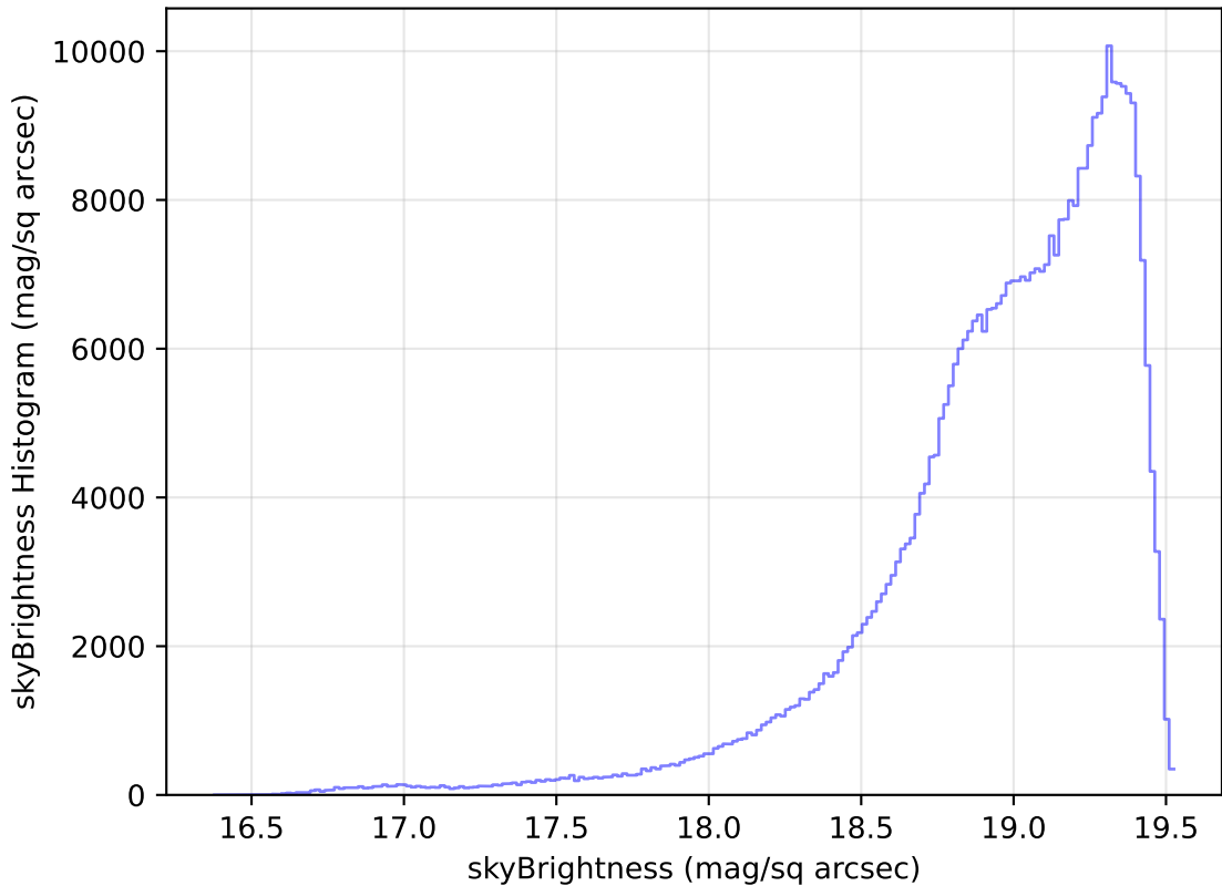
ddf_loaded_fl4_v3.4_10yrs All sky z band: skyBrightness Histogram
