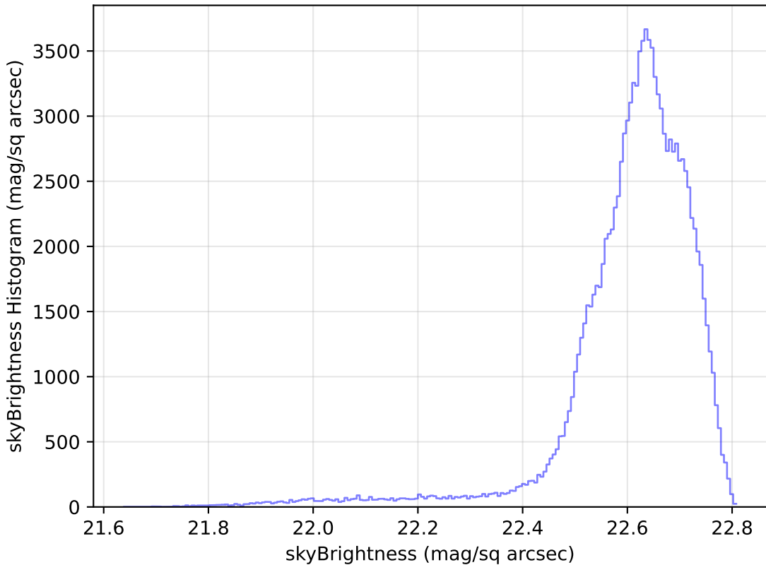
ddf_loaded_fl4_v3.4_10yrs All sky u band: skyBrightness Histogram
