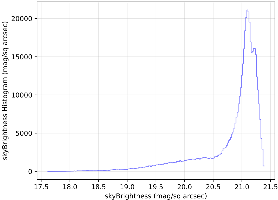
ddf_loaded_fl4_v3.4_10yrs All sky r band: skyBrightness Histogram
