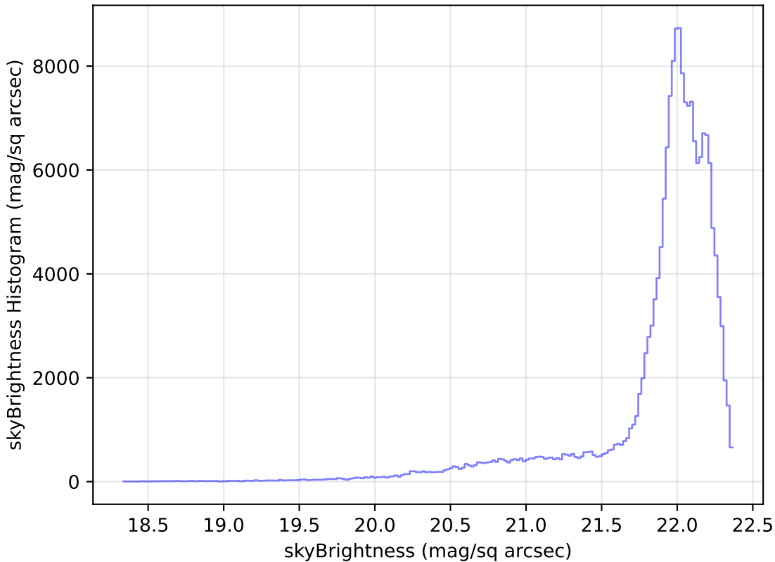
ddf_loaded_fl4_v3.4_10yrs All sky g band: skyBrightness Histogram
