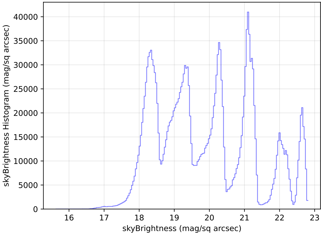
ddf_loaded_fl4_v3.4_10yrs All sky all bands: skyBrightness Histogram
