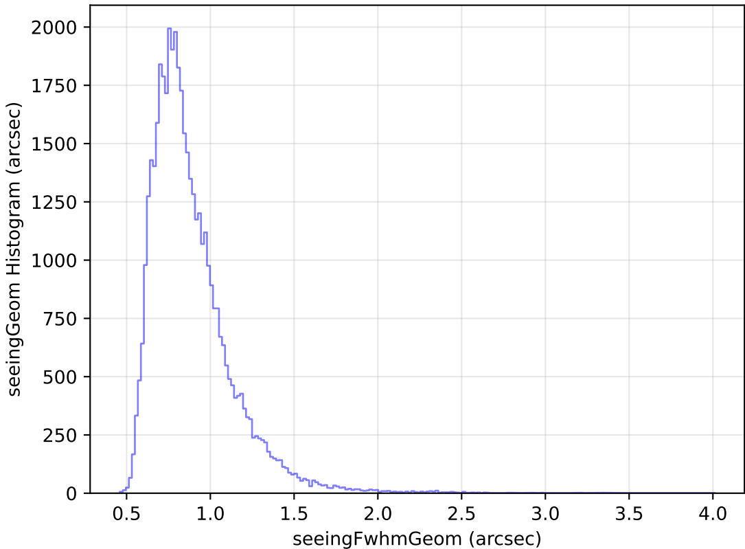
ddf_loaded_fl4_v3.4_10yrs Yr 1 z band: seeingGeom Histogram
