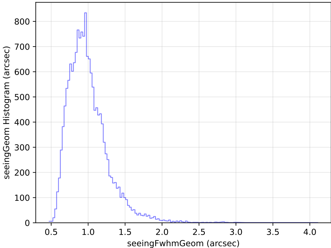
ddf_loaded_fl4_v3.4_10yrs Yr 1 u band: seeingGeom Histogram
