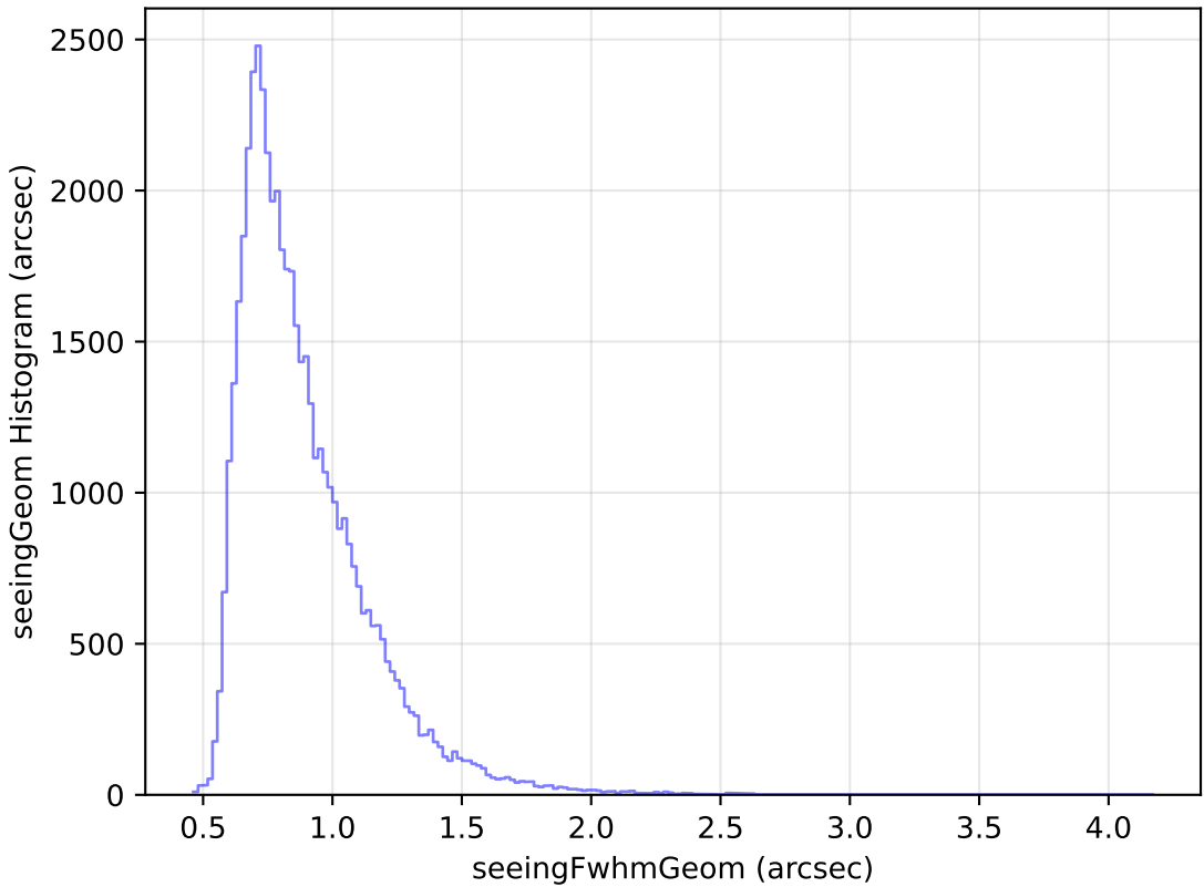
ddf_loaded_fl4_v3.4_10yrs Yr 1 r band: seeingGeom Histogram
