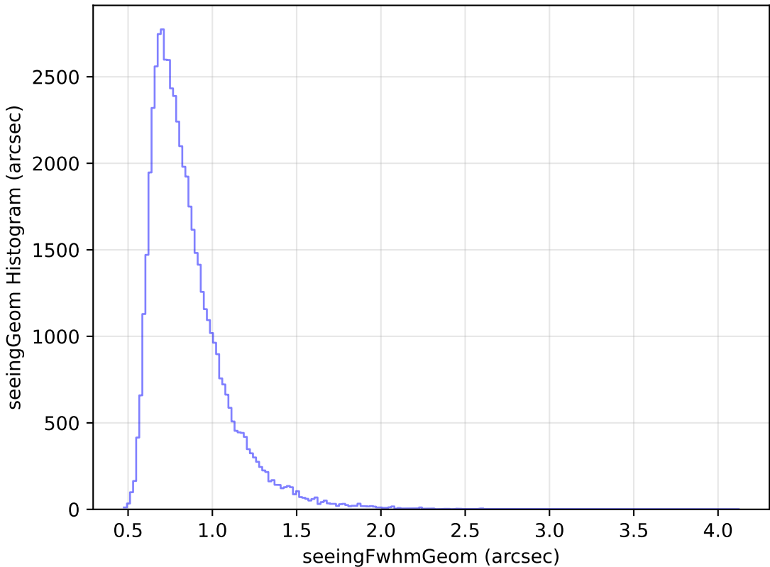
ddf_loaded_fl4_v3.4_10yrs Yr 1 i band: seeingGeom Histogram
