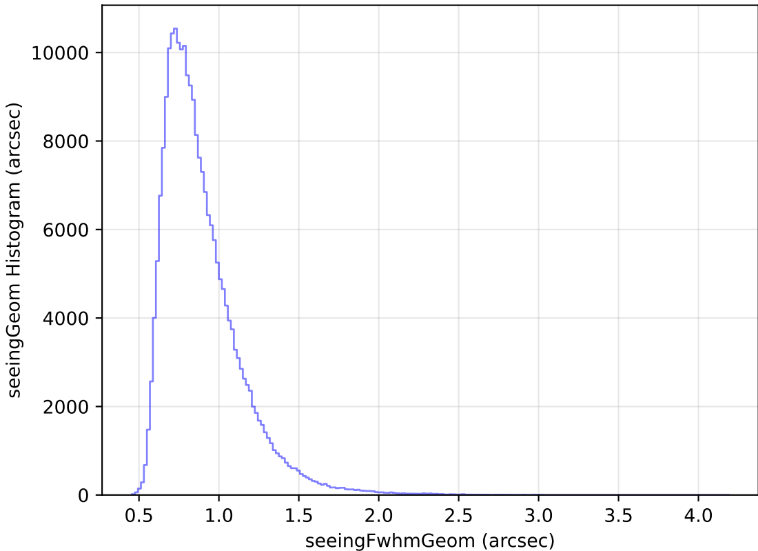
ddf_loaded_fl4_v3.4_10yrs Yr 1 all bands: seeingGeom Histogram
